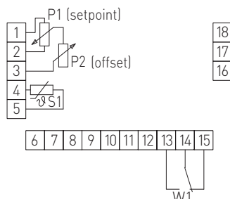
Connecting diagram
