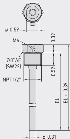
Dimensional drawing (inch)
