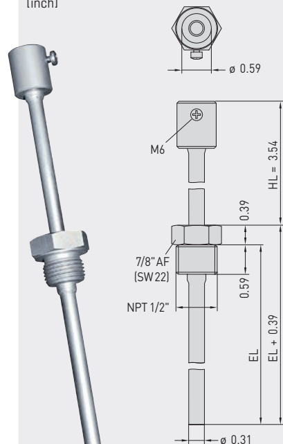
Dimensional drawing (inch)
